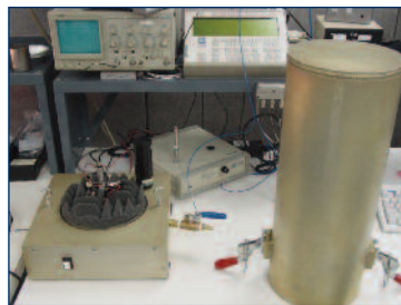
Microphone Electrostatic Calibration Test base & enclosure isolates unit under test from ambient noise and adjusts for barometric pressures, while voltage insertion generates excitation for comparative results
