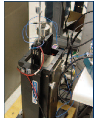
Low-frequency Accelerometer Calibrator 6" (152 mm) stroke shaker provides displacement for calibrations to 0.5 Hz
