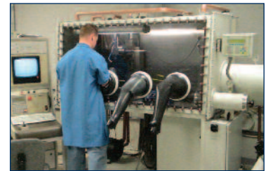
Glove box handling with laser welding permits inert gas to be added within the sensor
